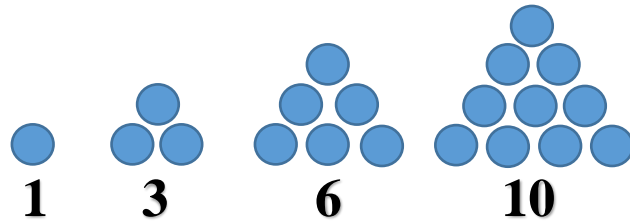
Figure 1: Triangular Numbers
